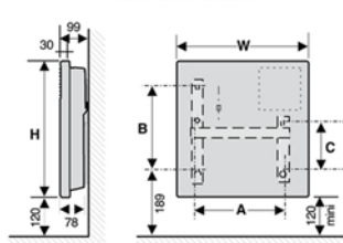
Installation scheme
